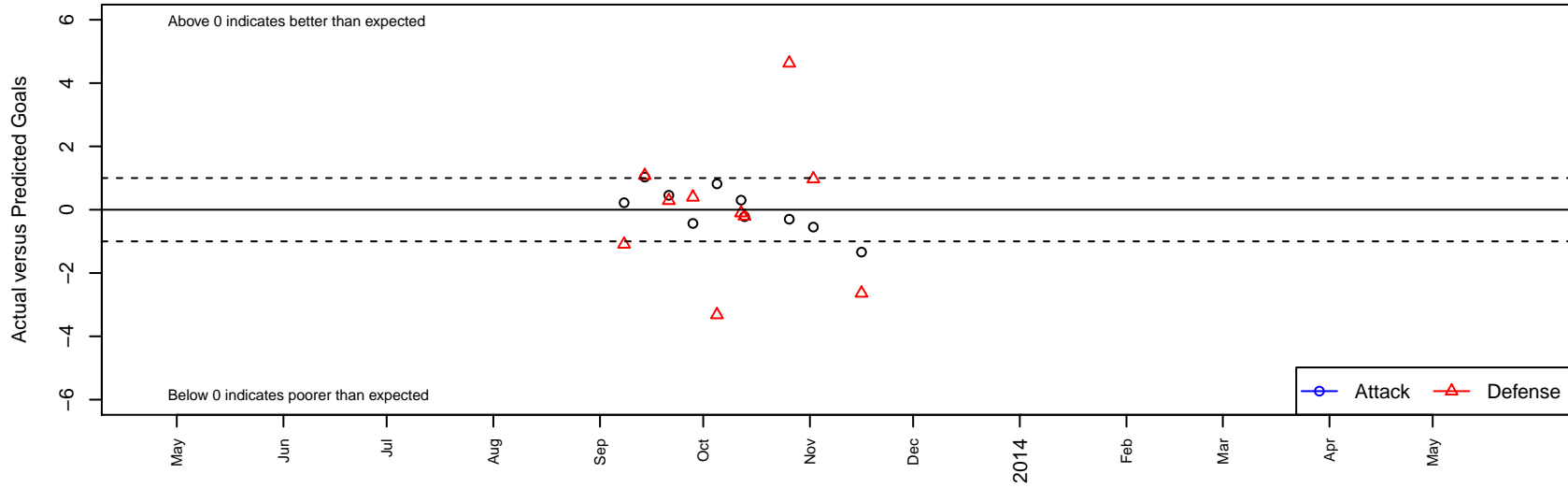
Beach FC Black G99 Dots are actual minus expected GF (blue circles) and GA (red triangles). Blue line is smoothed change in attack strength. Red is smoothed change in defense strength.
